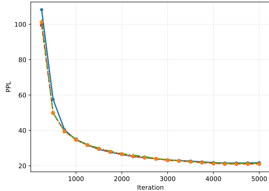
Validation PPL
