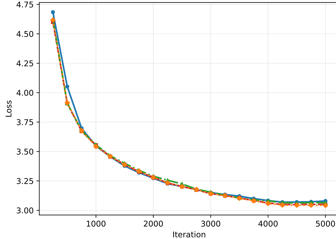
Validation Loss
