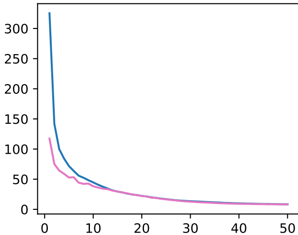
Jaccard
