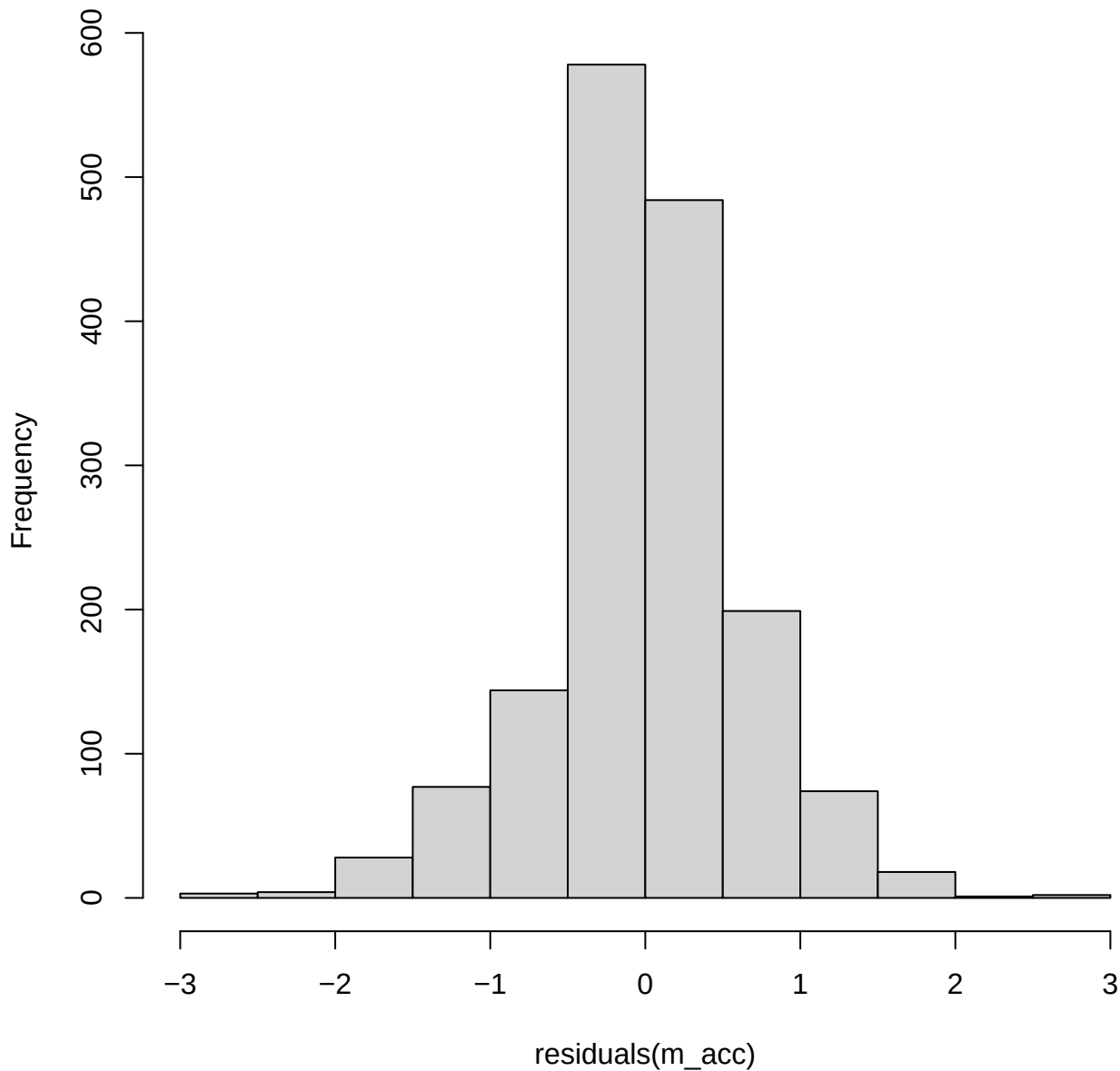
Histogram of residuals(m_acc)
