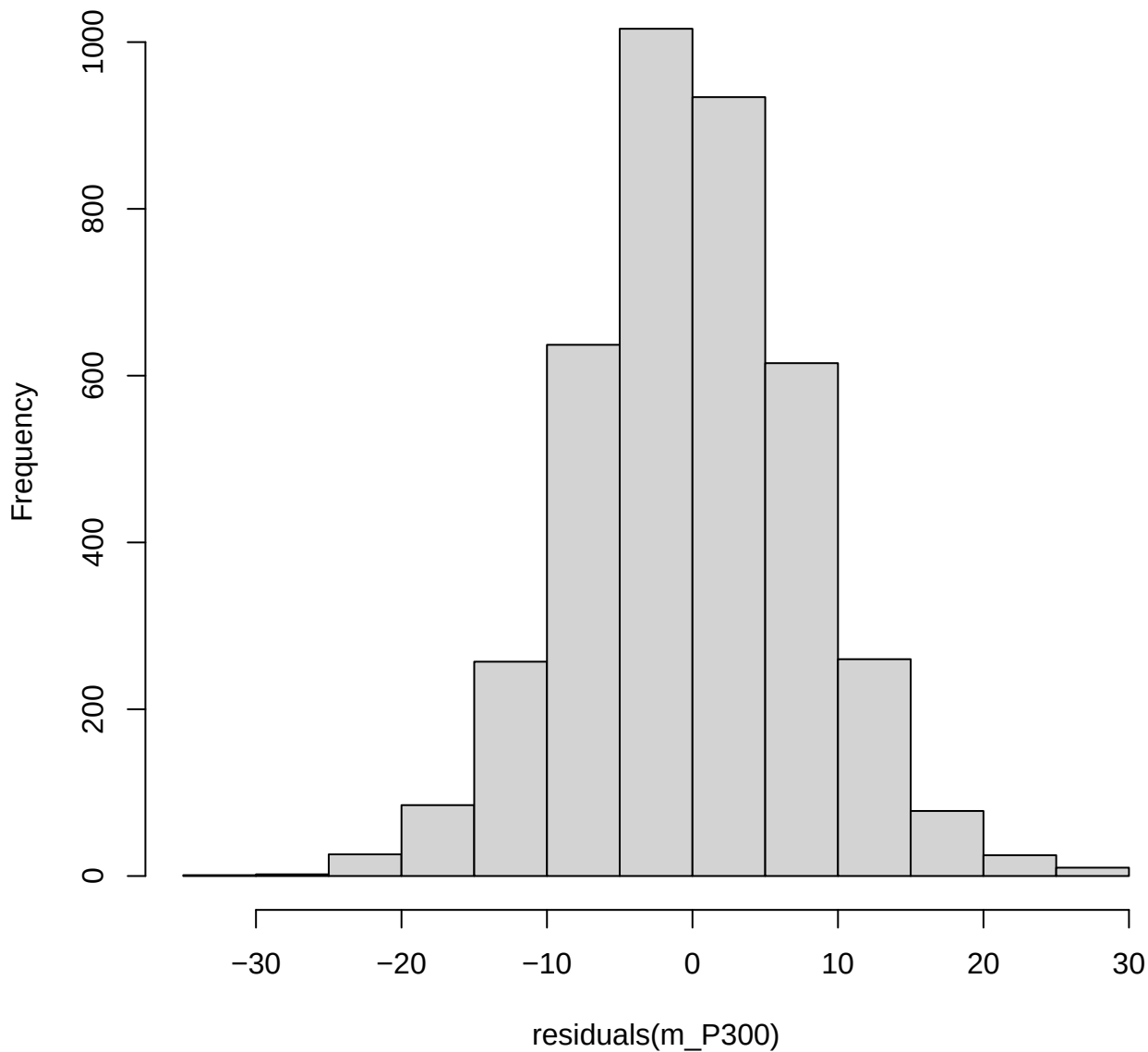
Histogram of residuals(m_P300)
