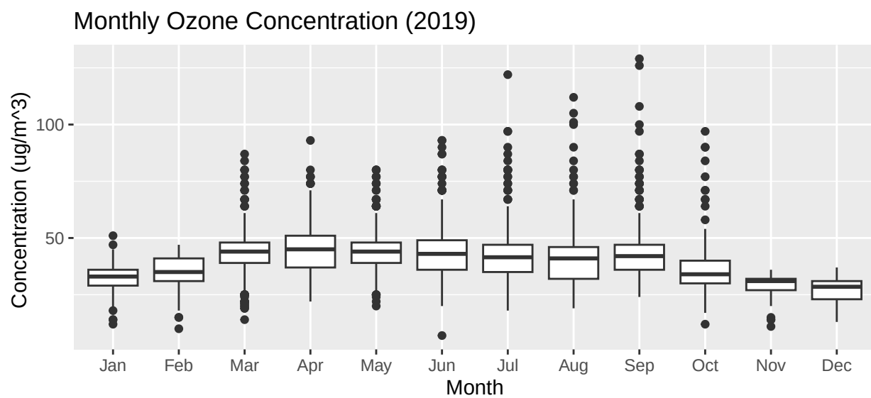
Figure 2: 2019 monthly Ozone level
