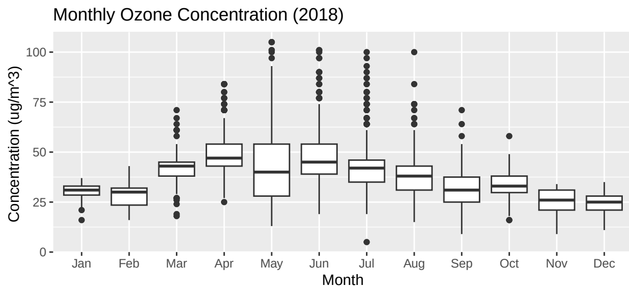
Figure 1: 2018 monthly Ozone level
