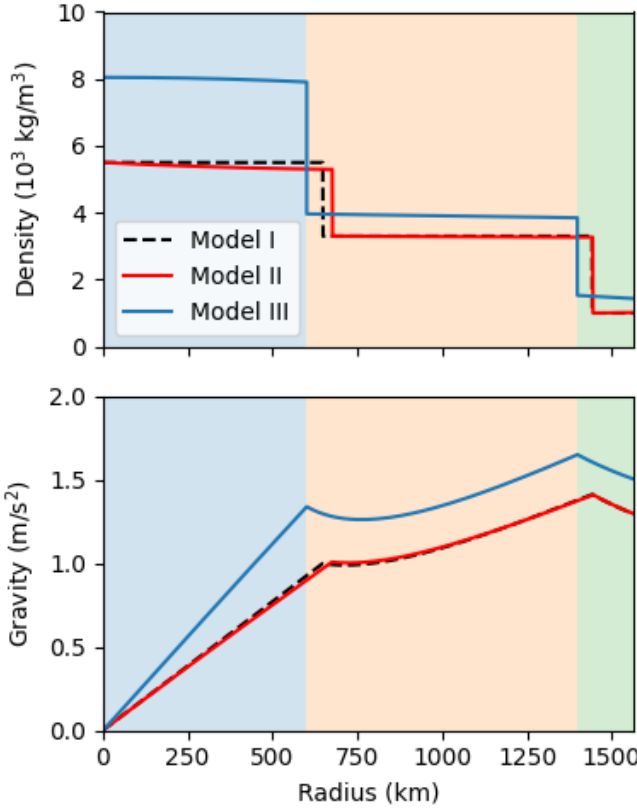
Figure 1: The density, pressure, gravity, and temperature profiles of Europa as calculated by the 3 different models.
