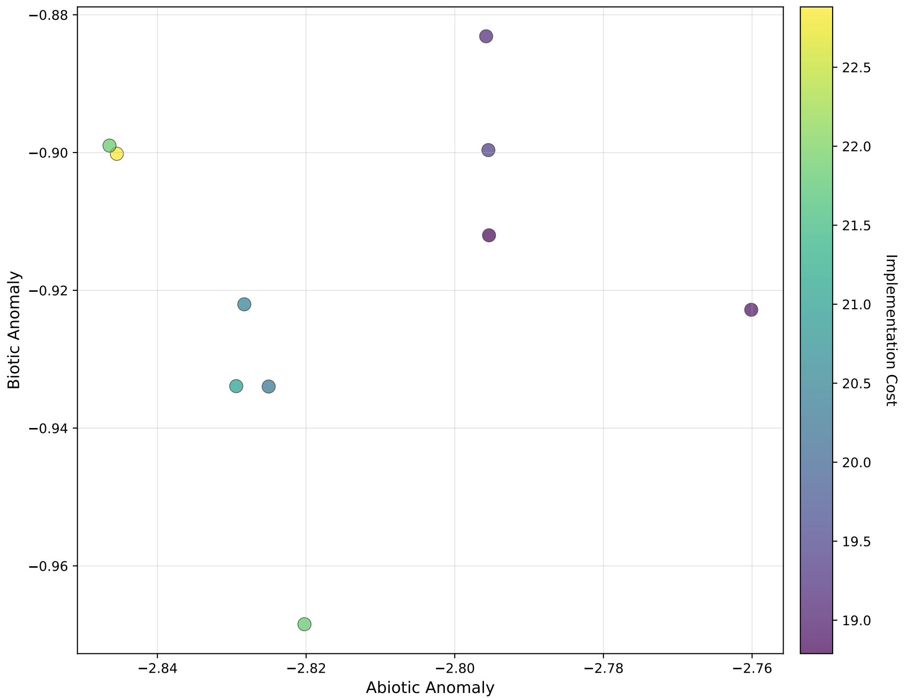
Pareto Front (10 solutions)
