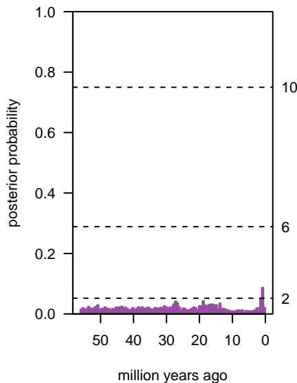
speciation shift times
