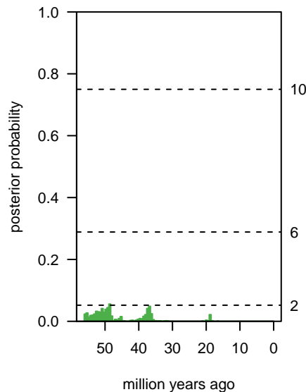
mass extinction times
