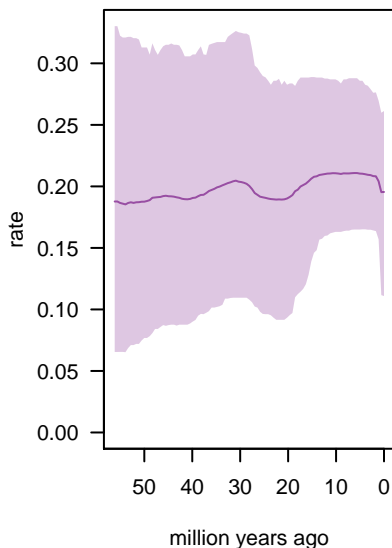
speciation rates
