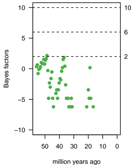
mass extinction Bayes factors
