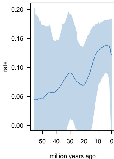
net-diversification rates
