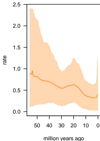
relative-extinction rates
