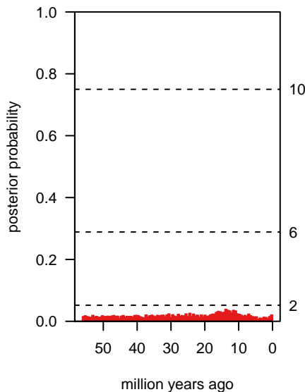
extinction shift times
