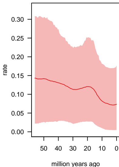
extinction rates
