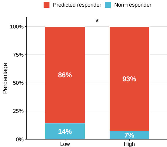
BLCA TIDE-predicted response
