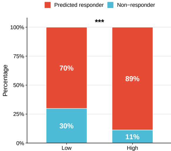
LUAD TIDE-predicted response
