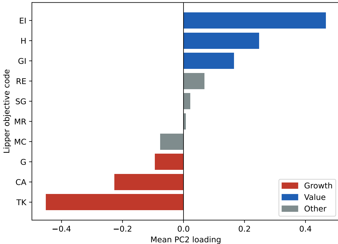
PC2 loading sorts by style mandate
