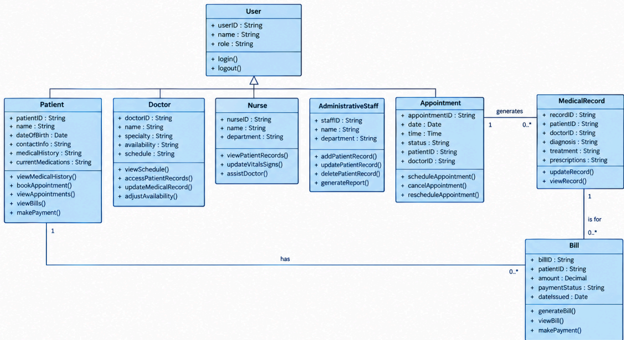
UML Class Diagram – Hospital Management System (HMS)
