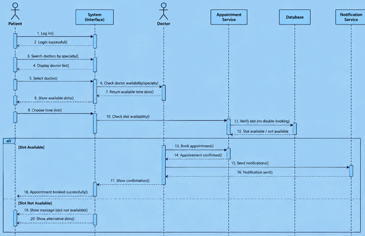
UML Sequence Diagram – Booking an Appointment
