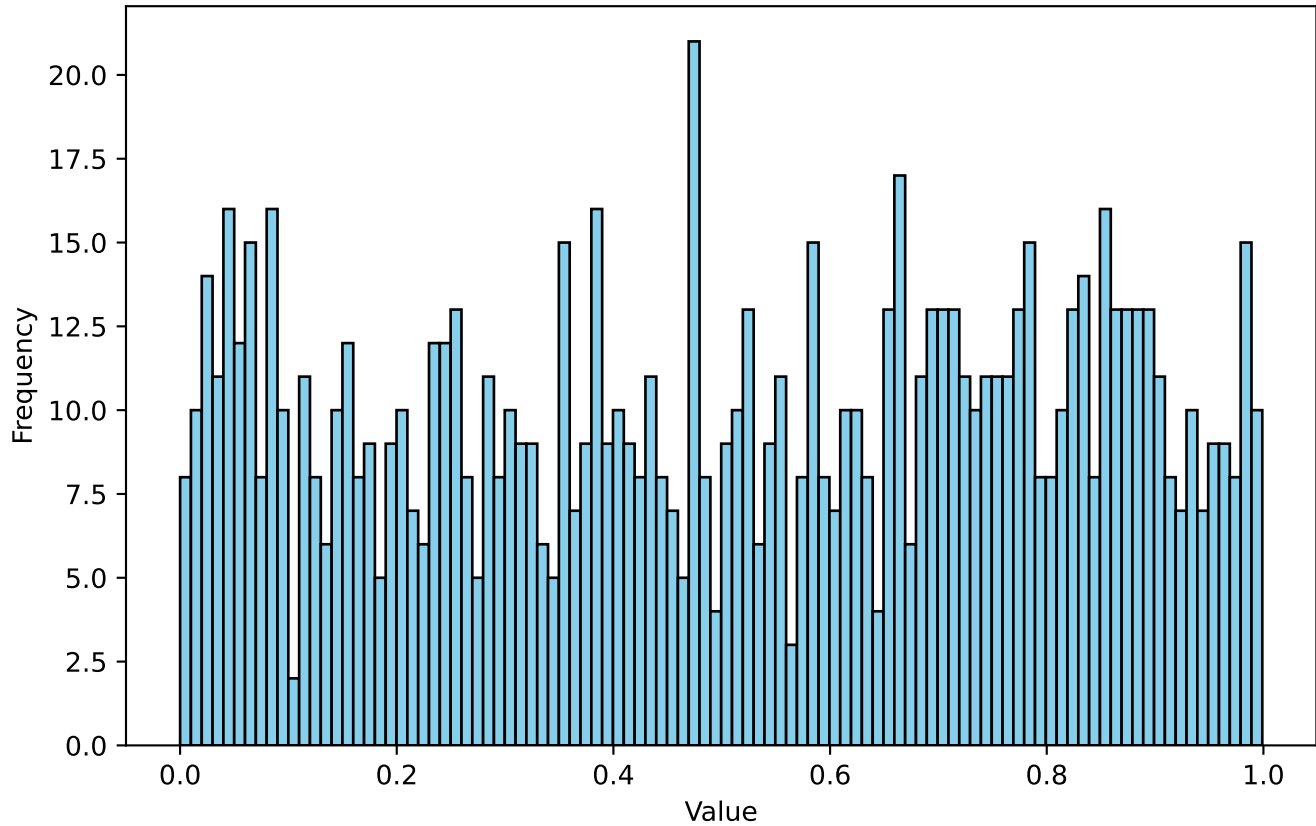
Histogram of 1000 Uniform Random Numbers
