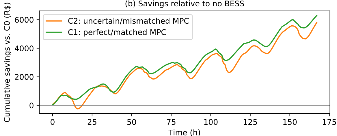
(b) Savings relative to no BESS
