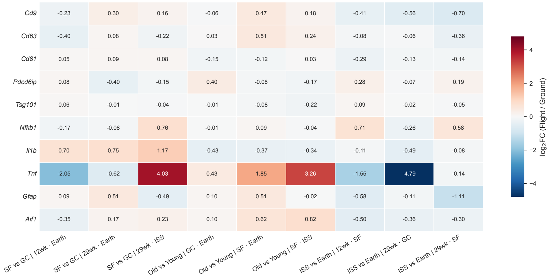
OSD-562 Hippocampus — focus-gene log 2 FC across all clean contrasts
