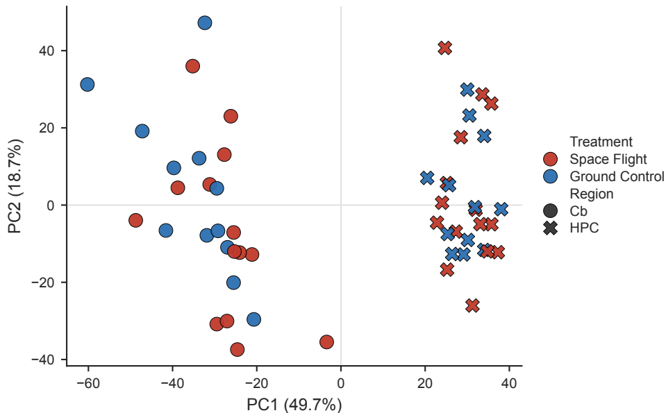
Combined Cb + HPC — PCA (coloured by treatment)
