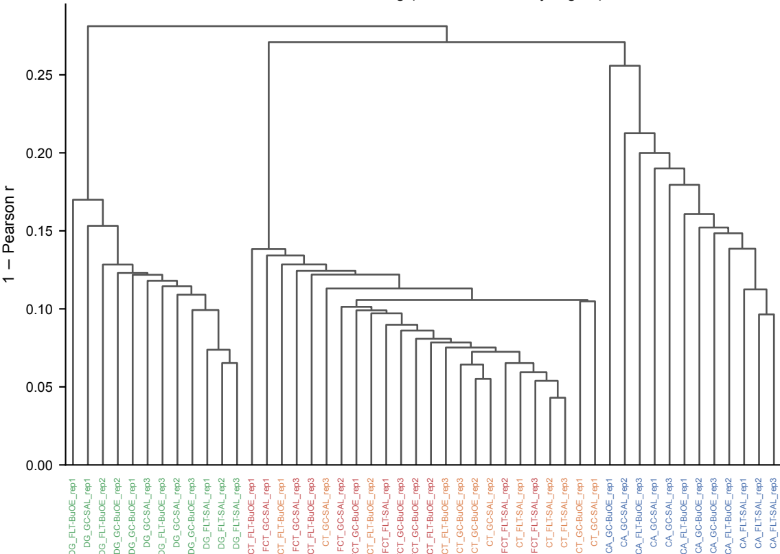
Hierarchical clustering (labels coloured by region)
