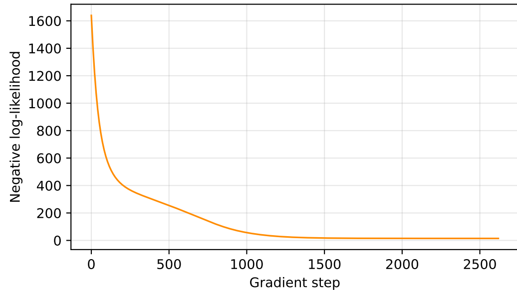
FullGP training curve
