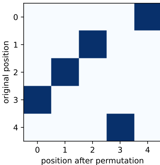
REPAIR estimate \hat{\pi}_X (hard)
