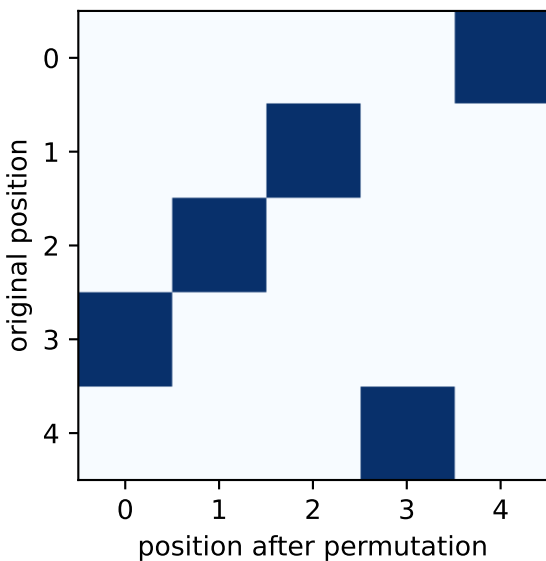
True \pi_X
