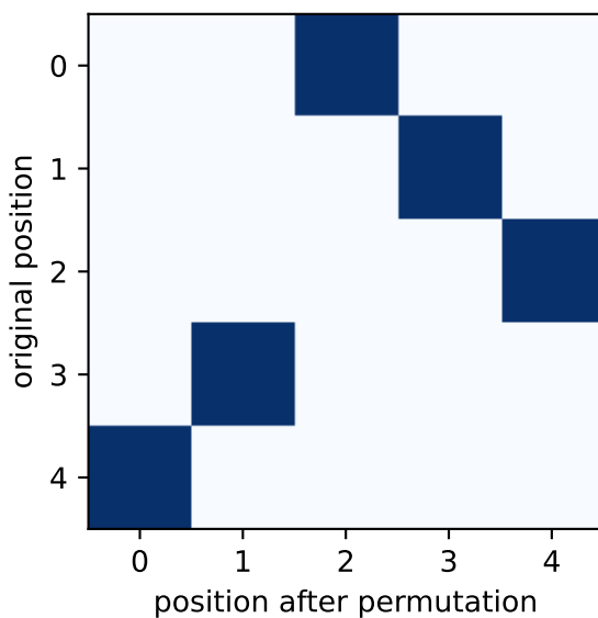
REPAIR estimate \hat{\pi}_S (hard)
