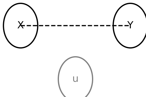
(D) This paper: unlinked linear models with dependent data
