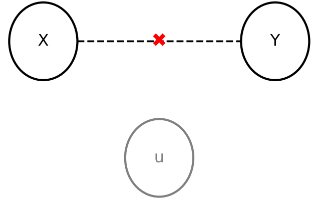
(D) This paper: unlinked linear models with dependent data
