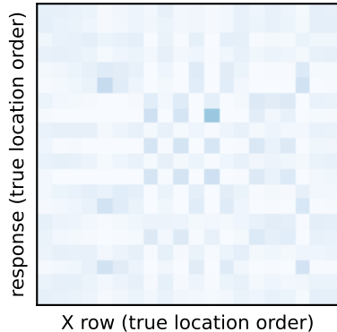
both keys, \beta=1.0 P(\text{true pairing}) = 0.10
