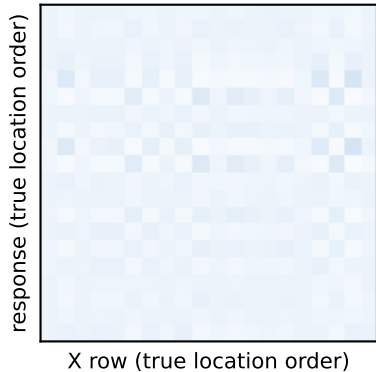
covariate key only, \beta=0.5 P(\text{true pairing}) = 0.06
