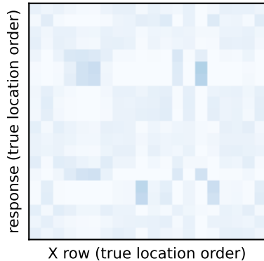
covariate key only, \beta=1.0 P(\text{true pairing}) = 0.08
