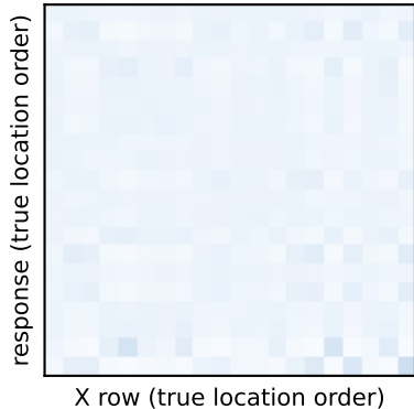
both keys, \beta=0.5 P(\text{true pairing}) = 0.07
