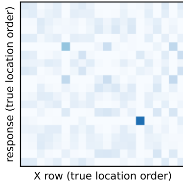
both keys, \beta=2.0 P(\text{true pairing}) = 0.13
