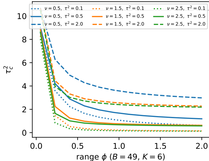
(b) \tau_C^2 vs range and nugget ( \sigma^2 = 5 )
