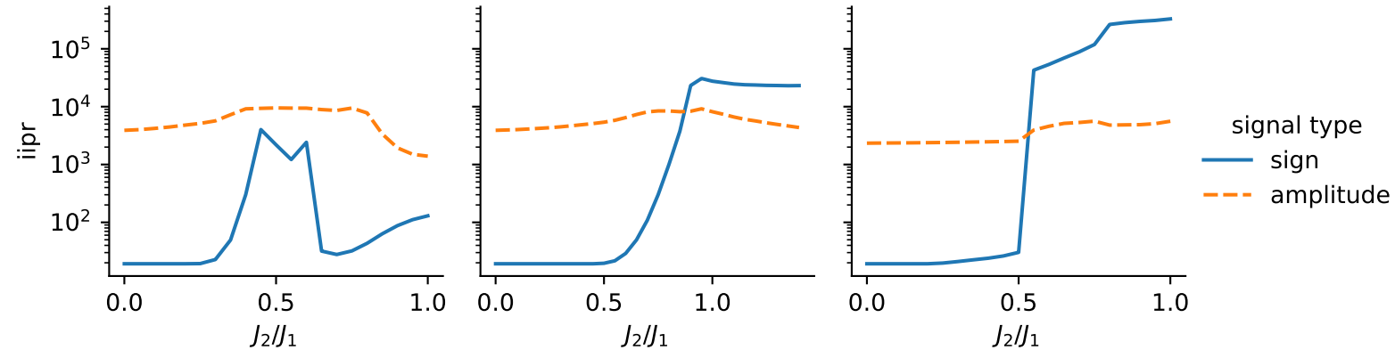
lattice = Square
