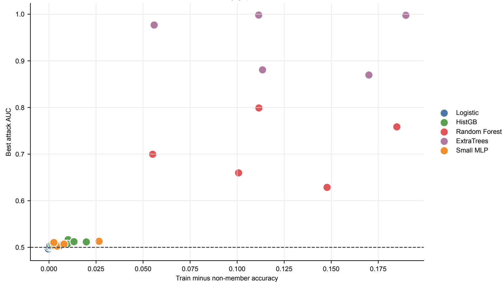
Train/non-member accuracy gap and best MIA AUC
