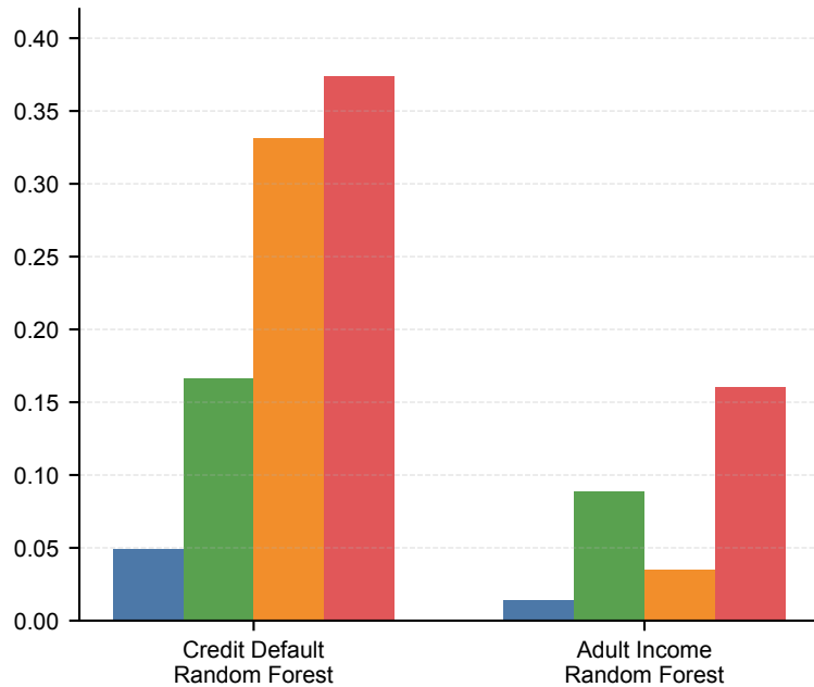
TPR@1%FPR
