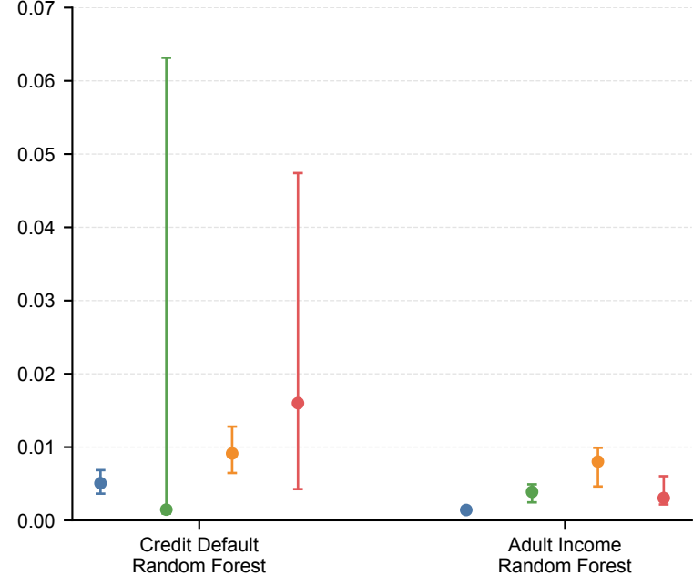
TPR@0.1%FPR
