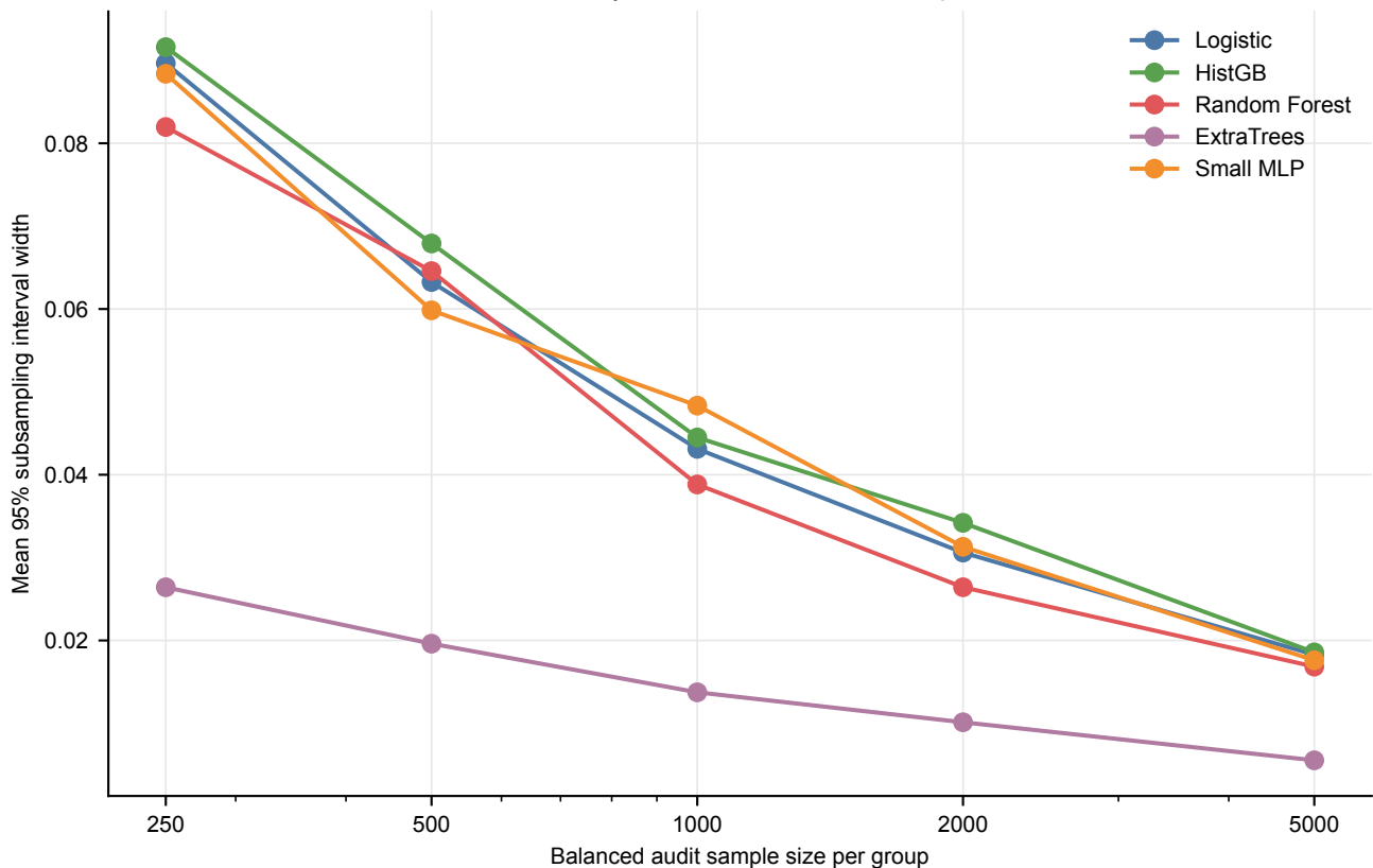
AUC variability decreases with audit sample size
