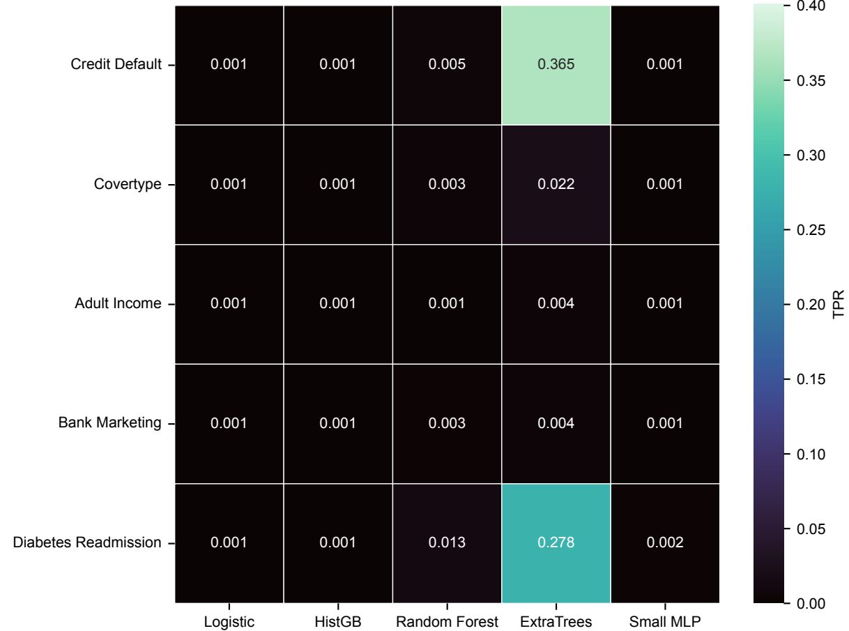
Negative-loss TPR at 0.1% FPR
