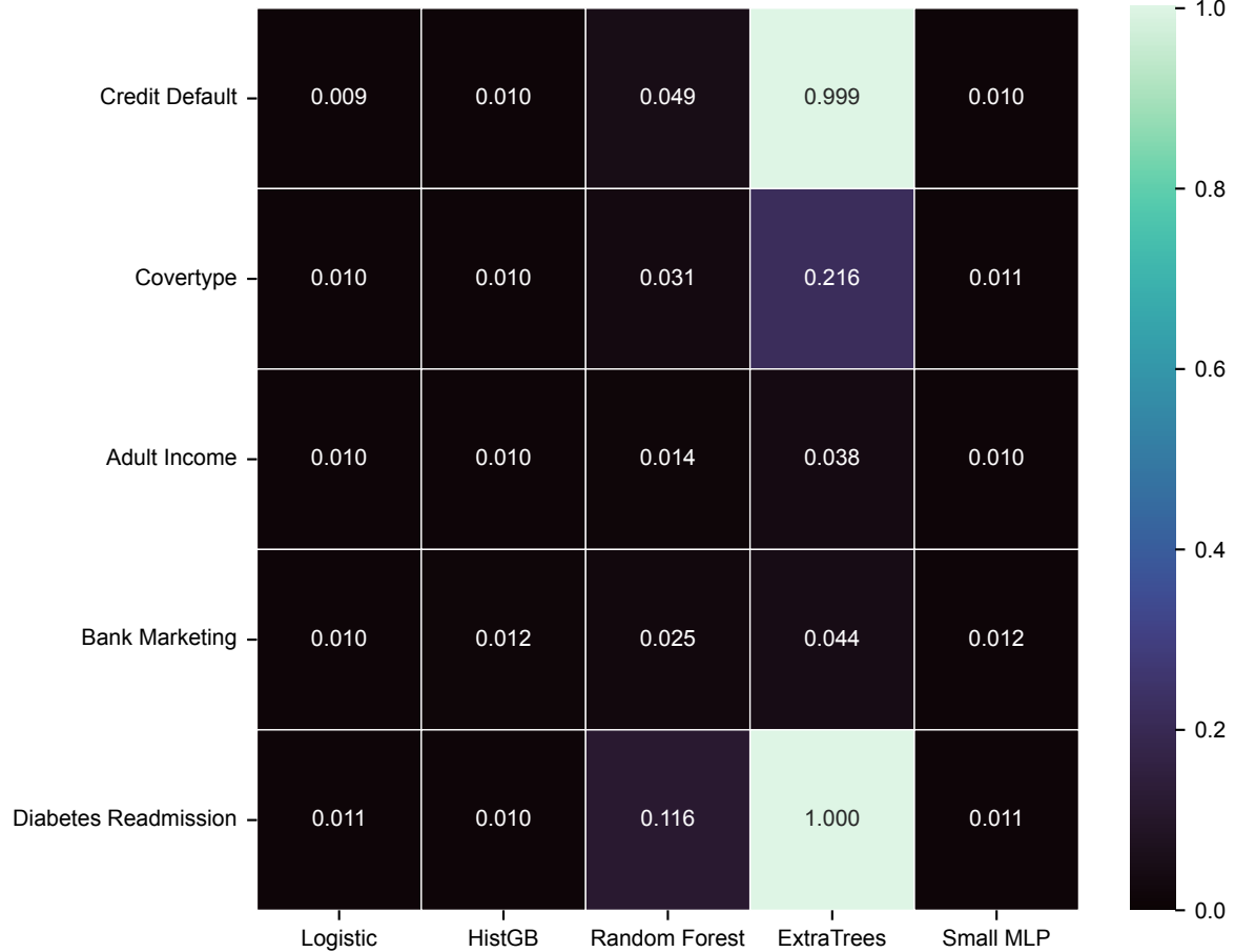
Negative-loss TPR at 1% FPR
