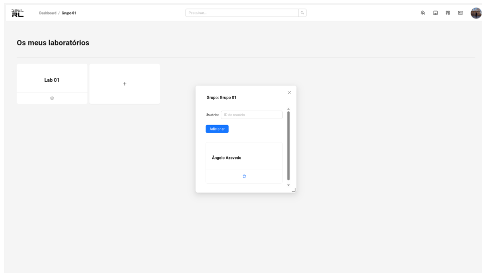
Figure 5.16: User management interface within a group, allowing professors to add, remove, and manage group members.
