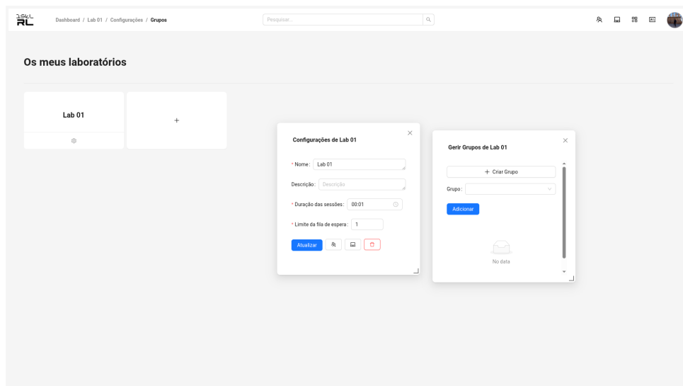
Figure 5.13: Group management interface for laboratories, showing existing groups and management options. This can be accessed both within specific laboratories and through the general management interface.
