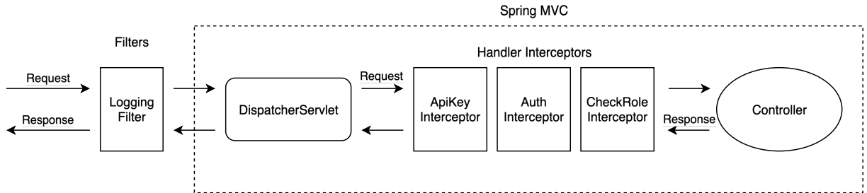
Figure 4.3: Implemented filters and interceptors.
