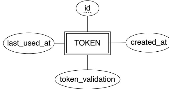
Figure 3.2: Token Entity
