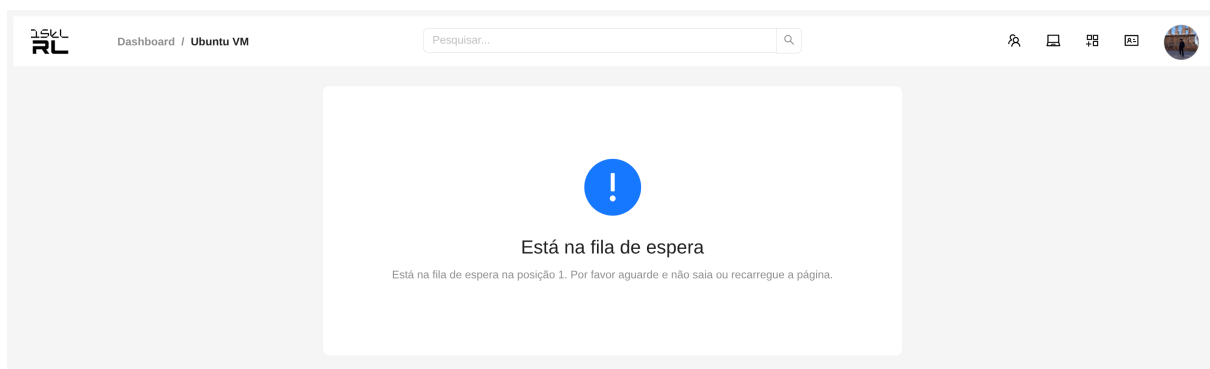
Figure 5.17: Waiting queue
