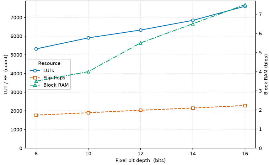
Figure 7: Resource usage vs pixel bit depth ( \text{MAX\_IMAGE\_WIDTH} = 12288 ).
