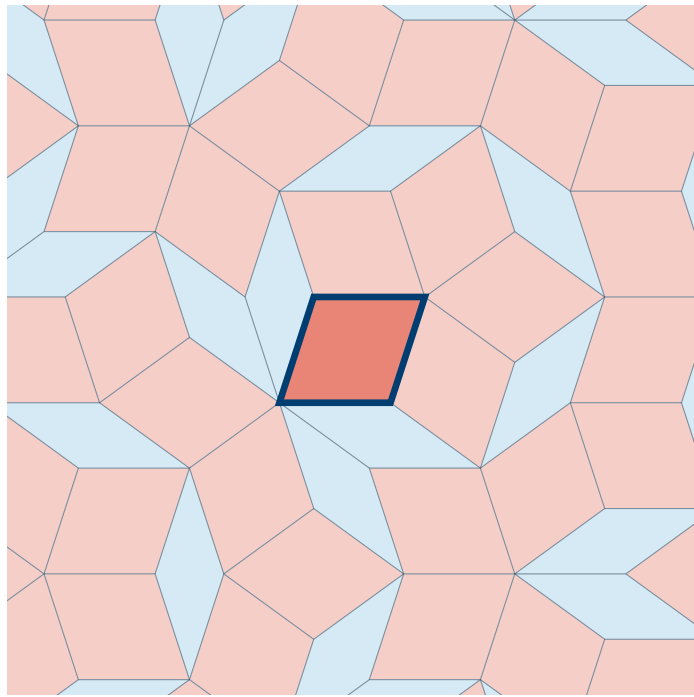
The corresponding thick rhombus
