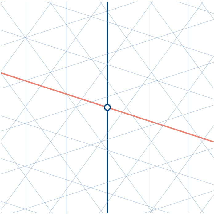
Grid lines L_0(1) and L_1(-2)
