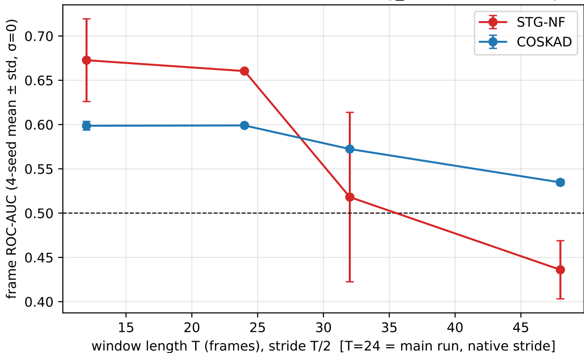
E2-window — MoCoDAD excluded (native seg_len 6 architecturally fixed)
