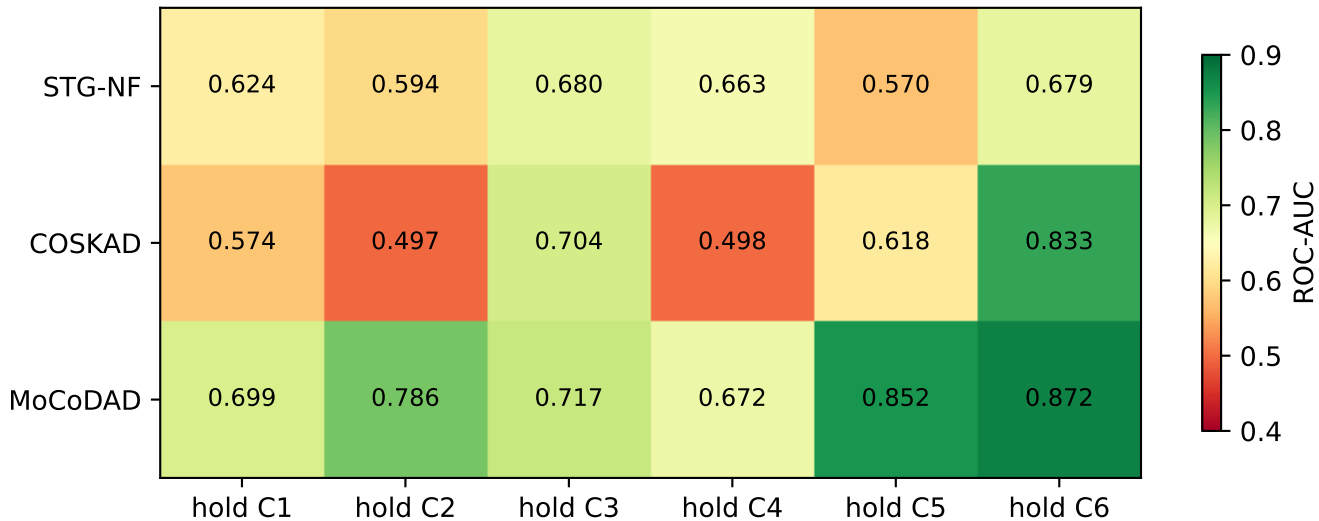
E1 — leave-one-camera-out frame ROC-AUC (4-seed mean, \sigma=0 )
