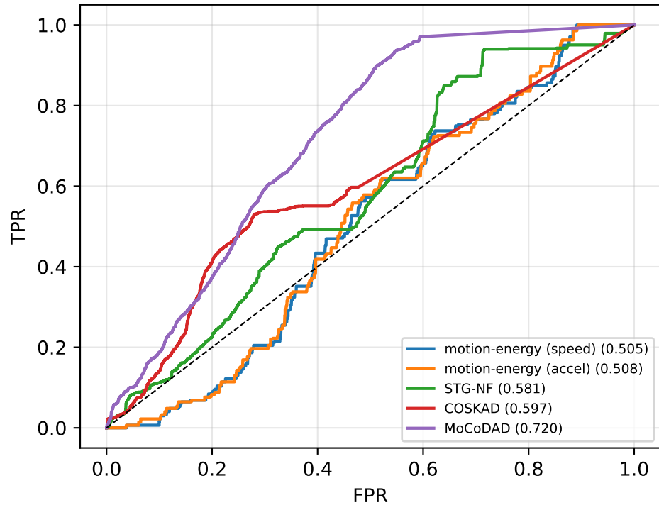
ROC — split (b) test, n=1, sigma=0
