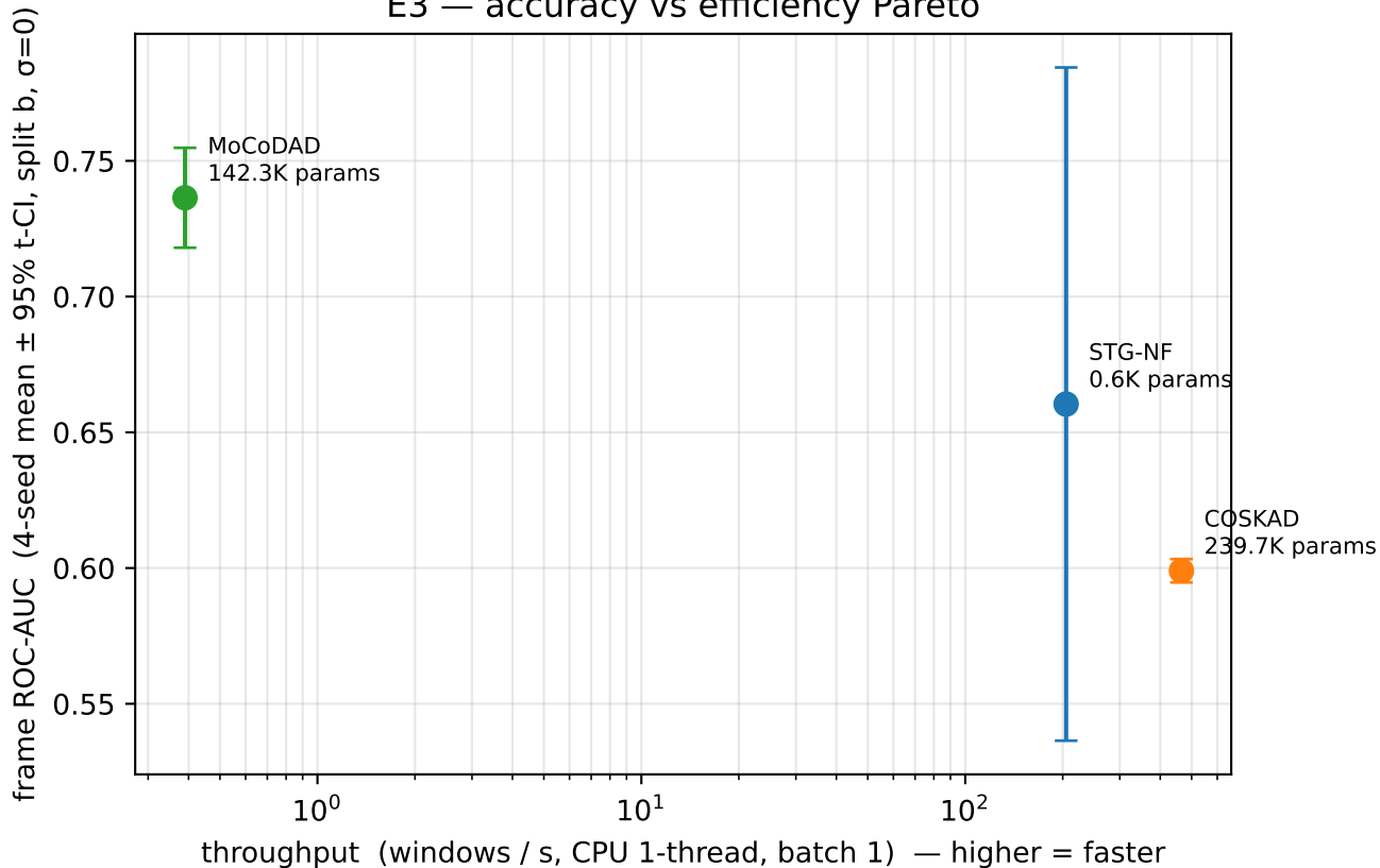
E3 — accuracy vs efficiency Pareto
