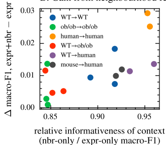
B. Gain from neighbourhood features
