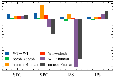
B. GraphSAGE – expr
