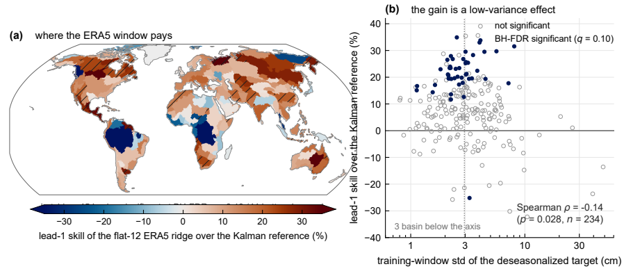
Figure 5. Where the forcing window helps. (a) Per-basin lead-1 skill (%) of the ERA5 flat-12 ridge over the Kalman reference on the 234 basins; basins significant under Benjamini–Hochberg false-discovery-rate control at q = 0.10 are hatched. (b) The same skill against each basin’s training-window storage standard deviation in centimeters of equivalent water height. The gain concentrates in low-variance basins.
