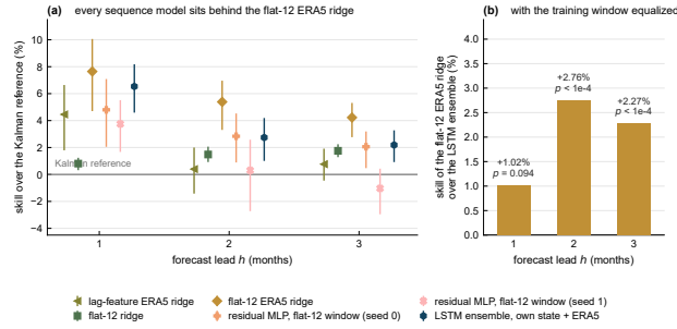
Figure 6. Sequence models against the flat ridge. Skill (%) over the Kalman reference at leads 1 to 3 for the LSTM ensemble, the residual MLP, the ERA5 lag ridge and the two flat-12 ridges, with the equalized-training-window comparison in which the ERA5 flat-12 ridge is refit on the LSTM’s exact training rows. Every sequence model sits below the linear reader of the same twelve-month history.
