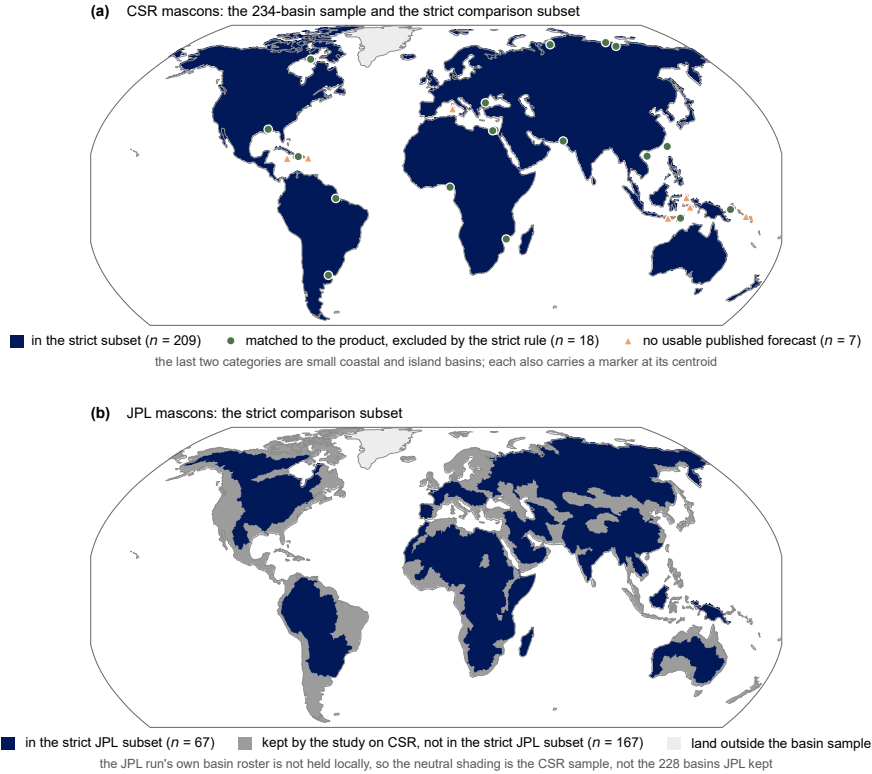
Figure 1. The basin sample. (a) The 234 basins kept on the CSR product, colored by membership in the strict comparison subset of Sect. 3.6: 209 basins enter the comparison with the published product, 18 are matched to that product but fail the full-containment rule, and 7 have no usable cell of the product at all. (b) The same on the JPL product, where 67 basins pass the rule.
