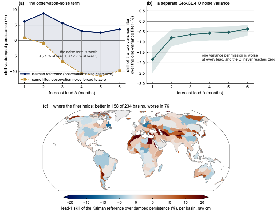
Figure 4. Why the filter wins. (a) Skill lost when the observation-noise term is removed from the filter, by lead: the noise-free filter against the Kalman reference. (b) The mission-split filter against the single-variance filter by lead; negative means the split hurts. Both panels carry moving-block bootstrap 95 % confidence intervals. (c) Per-basin lead-1 skill of the Kalman reference over the stronger damped-persistence variant on the 234 basins.
