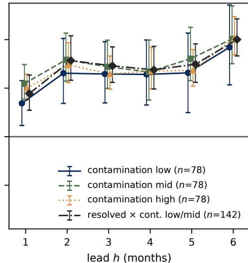
(b) stacked correction (LSTM ens.)
