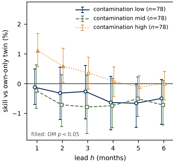
(a) linear arm (ridge, +ERA5)
