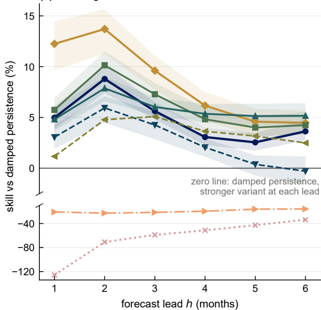
(a) skill against the conventional reference
