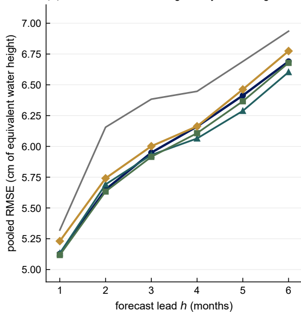
(b) the same models weighted by raw storage
