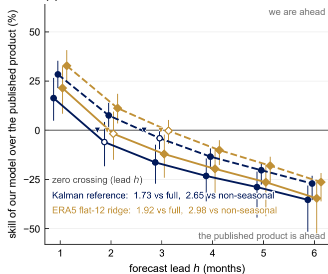
(a) CSR mascons, 209 basins, 60 months
