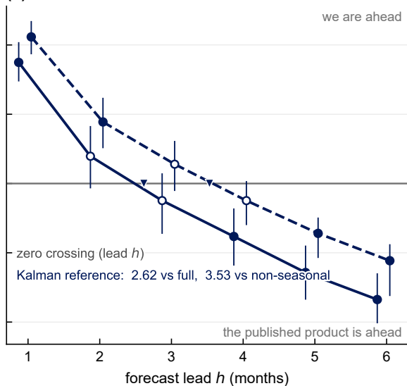
(b) JPL mascons, 67 basins, 59 months
