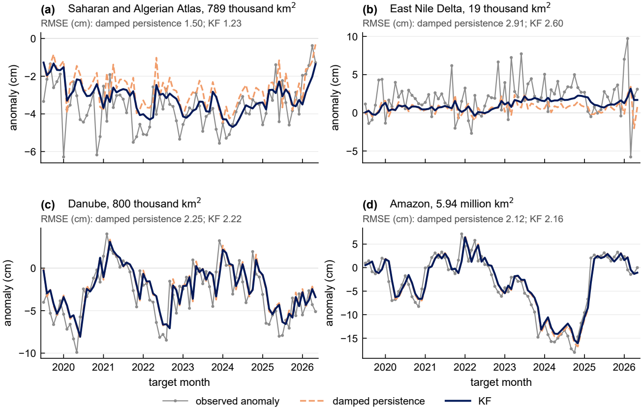
Figure 3. Observed deseasonalized storage anomaly (grey) and the 1-month forecasts of damped persistence ( \rho^h variant, dashed) and KF (solid) in four basins, in centimeters of equivalent water height, over the full test window. The panels span the range of per-basin outcomes at a 1-month lead time: (a) and (b) two arid basins with noisy observations, where the filter gains most; (c) a mid-latitude river basin where the gain is a few percent; (d) the Amazon, where damped persistence is marginally better. Each panel states the 1-month RMSE of both forecasts over the window.
