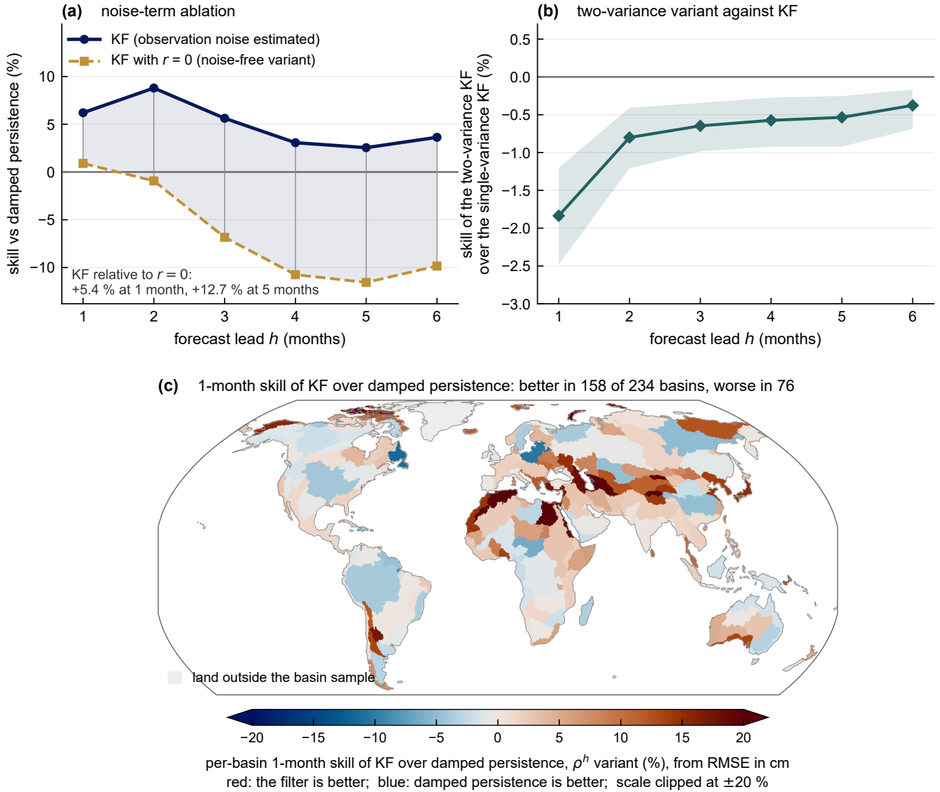
Figure 4. Attribution of the filter’s margin. (a) Skill (%) against the regression damped-persistence variant at every lead time for KF and for the noise-free variant (KF with r = 0 ). Shading shows the difference in skill relative to this common reference, without a confidence interval. The annotated improvement of KF relative to r = 0 uses the latter’s MSE as its denominator and therefore differs from the shaded vertical gap. Because the reference here is the regression variant at every lead time, KF has a skill of +6.21 % at a 1-month lead time rather than the +5.0 % of Table 2, which uses the stronger \rho^h variant at that lead time. (b) The two-variance variant against the single-variance KF by lead time, with moving-block bootstrap 95 % confidence intervals; negative means the split hurts. (c) Per-basin 1-month skill of KF over the \rho^h damped-persistence variant on the 234 basins, computed from RMSE in centimeters; KF is better in 158 basins and damped persistence in 76. The color scale is clipped at \pm 20 %, and land outside the basin sample is pale grey.
