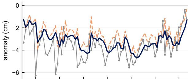
(a) Saharan and Algerian Atlas, 789 thousand km 2 1-month RMSE 1.50 cm (damped persistence), 1.23 cm (Kalman filter)
