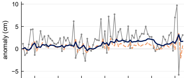
(b) East Nile Delta, 19 thousand km 2 1-month RMSE 2.91 cm (damped persistence), 2.60 cm (Kalman filter)
