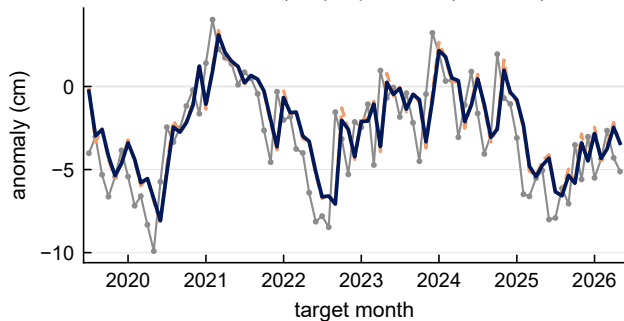
(c) Danube, 800 thousand km 2 1-month RMSE 2.25 cm (damped persistence), 2.22 cm (Kalman filter)
