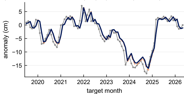
(d) Amazon, 5.94 million km 2 1-month RMSE 2.12 cm (damped persistence), 2.16 cm (Kalman filter)
