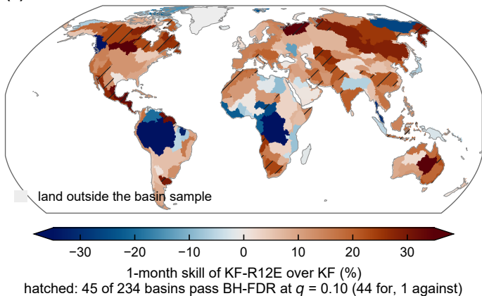
(a) 1-month skill of KF-R12E over KF
