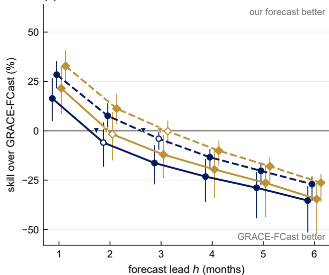
(a) CSR mascons, 209 basins, 60 months
