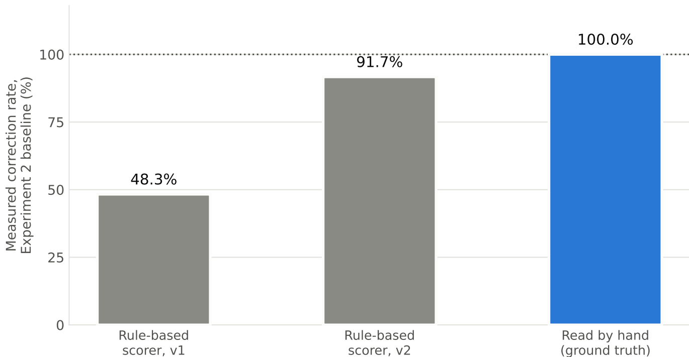
The same 60 responses, scored three ways
