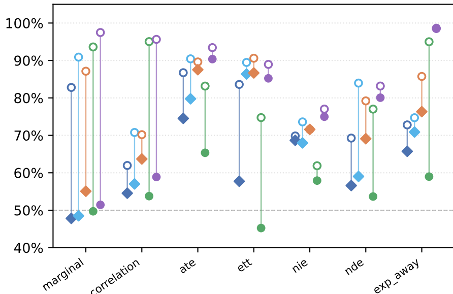
Accuracy by query type
