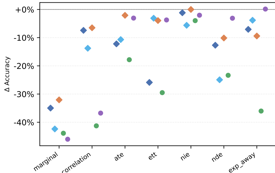
Accuracy change (96 – baseline)
