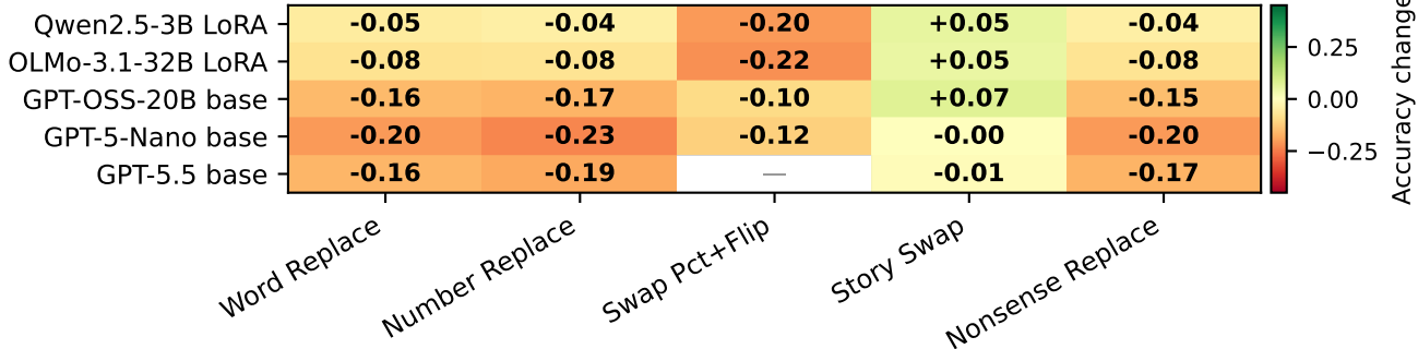
Accuracy change under intervention (all splits pooled)
